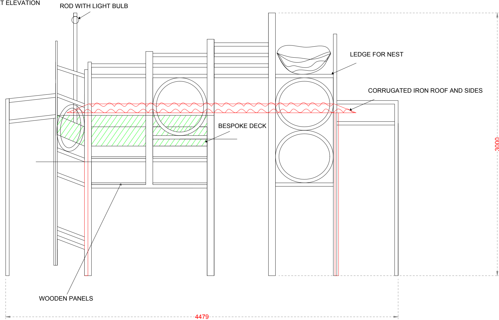
STEEL FRAME - FULL FRONT ON - FLAT ELEVATION
