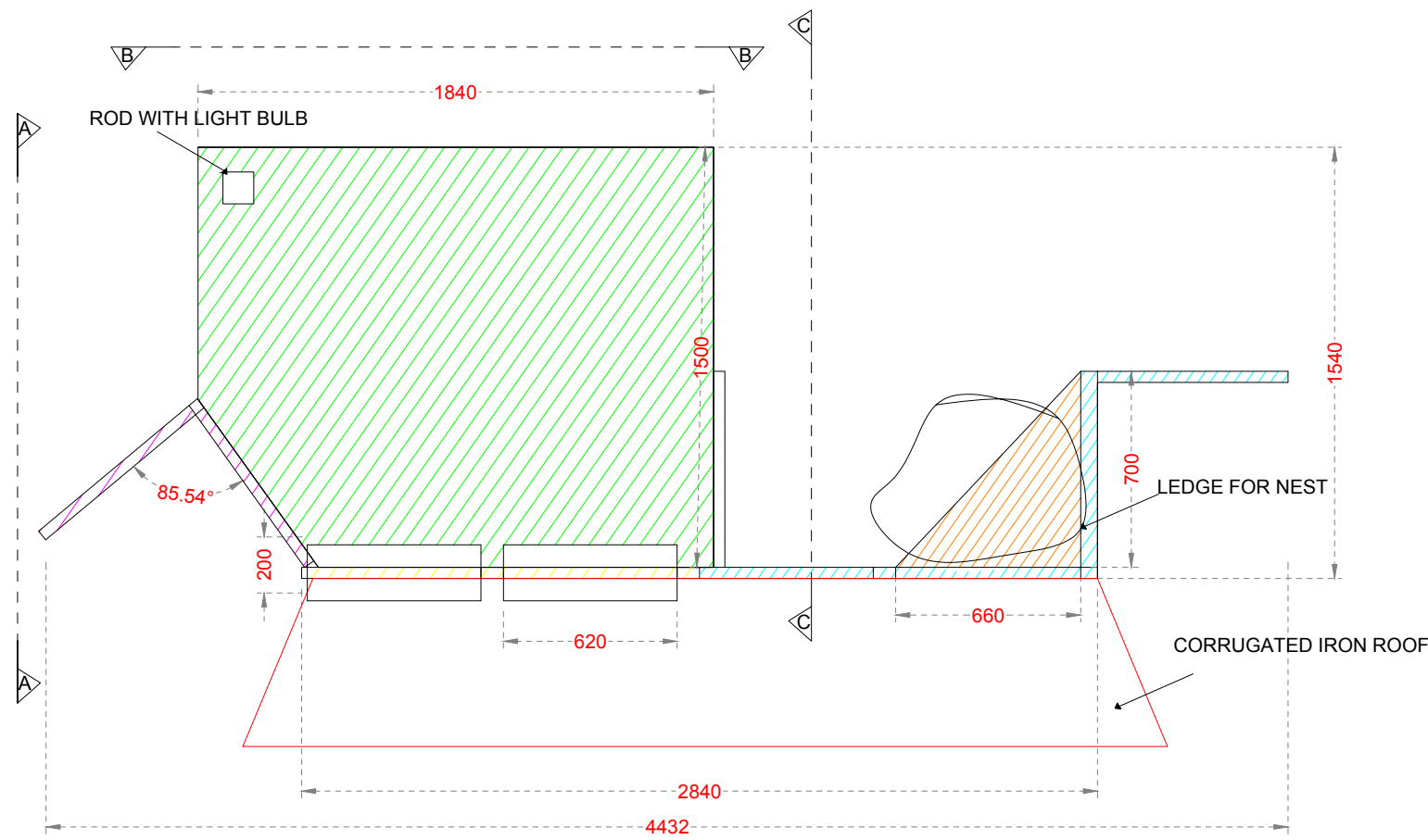
STEEL FRAME - FULL FRONT ON - FLAT ELEVATION
