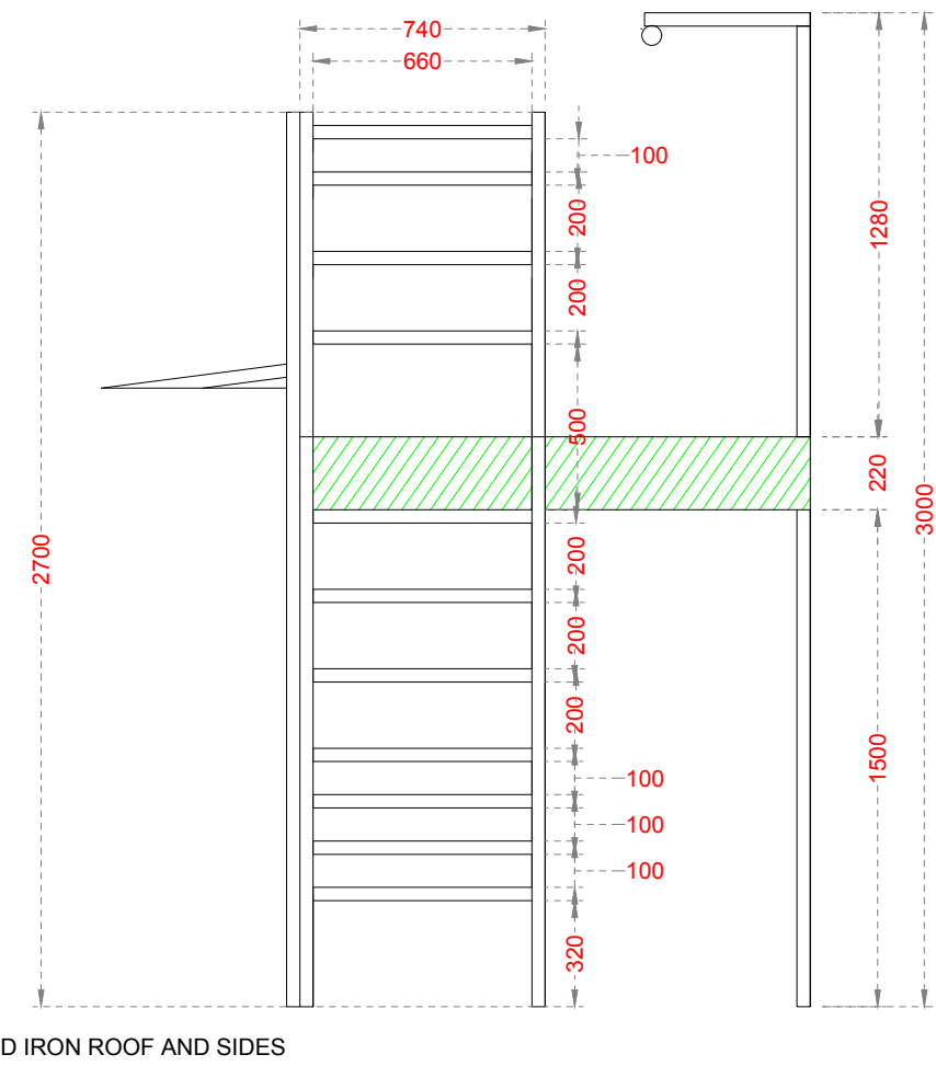
STAGE LEFT SECTION - C-C ELEVATION
